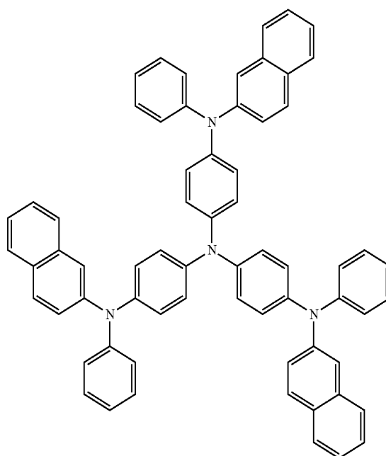
2-TNATA
